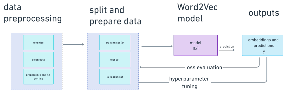
Figure 34: Steps for creating Word2Vec model
