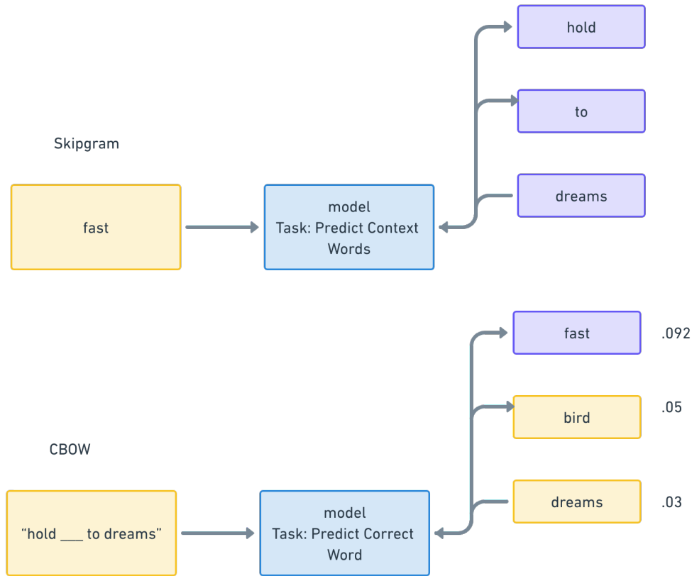
Figure 32: Word2Vec Architecture
